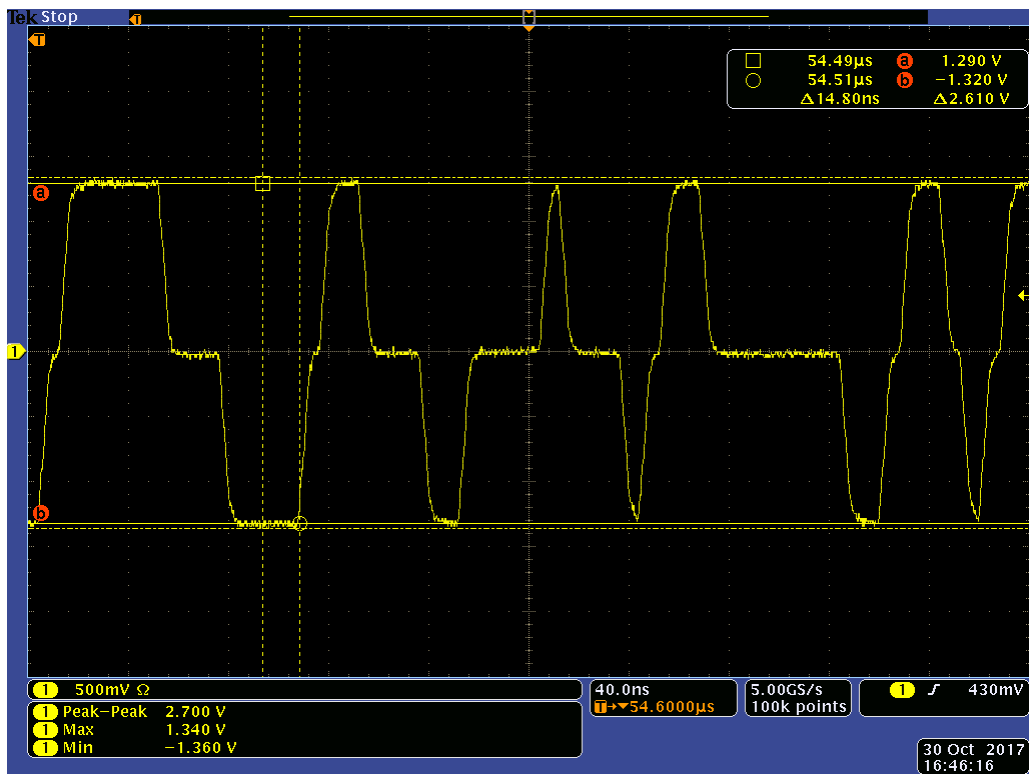
Figure 1: W5500 RX pins on custom PCB (Diff Probe)
