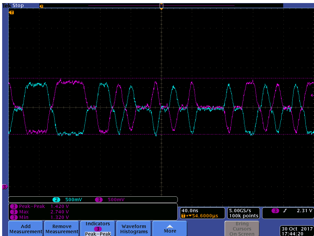
Figure 4: W5500 RX pins on Arduino Enet 2 Shield (2 single ended probes)
