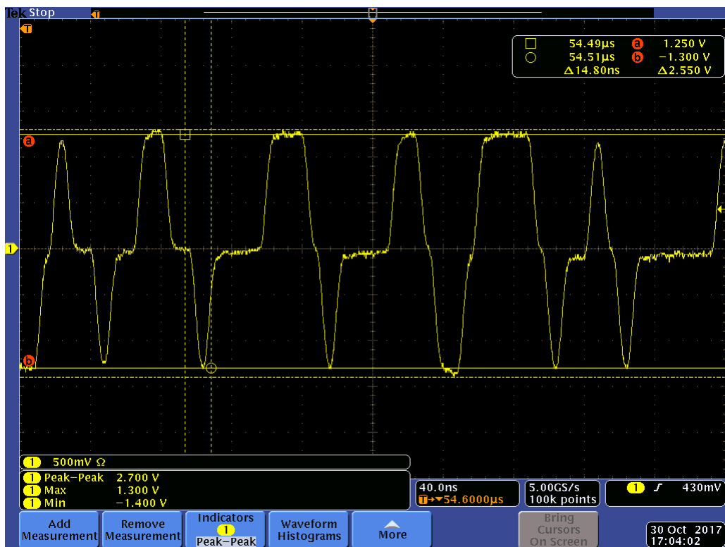
Figure 2: W5500 RX pins on Arduino Enet 2 Shield (Diff Probe)
