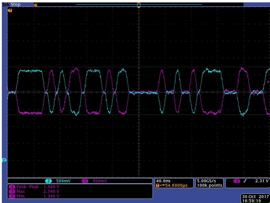
Figure 3: W5500 RX pins on custom PCB (2 single ended probes)
